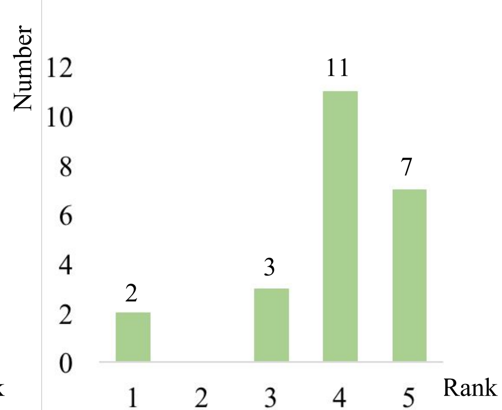
RetinexNet
